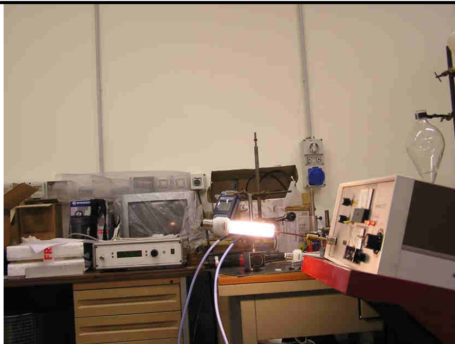
Fig.4: The commercial fluorescent lamp is on, fed with microwave power at 2.45 GHz.
